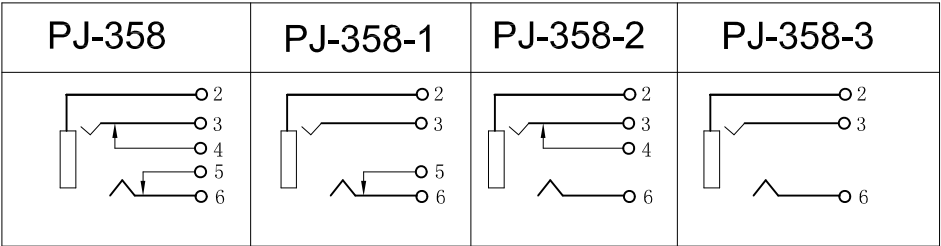
Circuit Schematic Diagram
