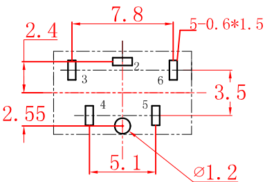
PCB Mounting Hole Dimensions
